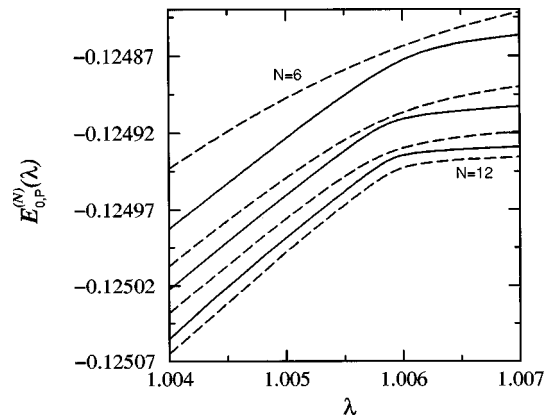
FIG. 8. Variational energy of the triplet ( 2p^2\ ^3P ) as a function of \lambda for N=6,7,\dots,12 . The dashed curves correspond to even values of N while the solid lines to odd values of N .
