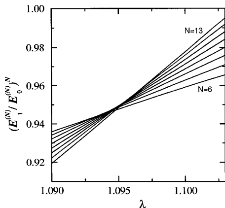
FIG. 1. The ratio between the ground-state energy and the second lowest eigenvalue raised to a power N as a function of \lambda for N=6,7,\dots,13 .
