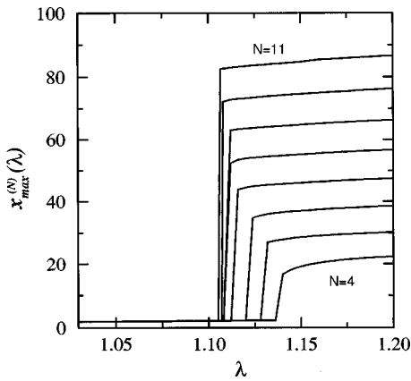
FIG. 6. Position of the highest maxima of the conditional probability P_\lambda(a_0|r) as a function of \lambda for N=4,5,\dots,11 .
